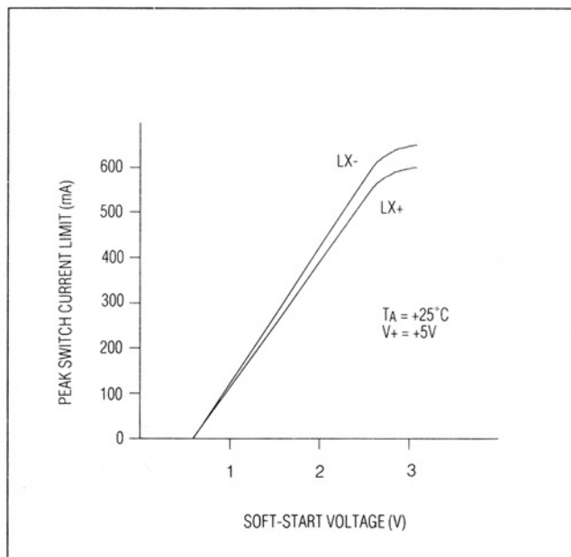
Figure 10. Typical Peak Switch Current Limit vs. Soft-Start Voltage
