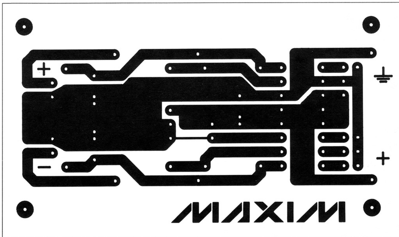
Figure 6. PC Layout for Circuit of Figure 4 Using MAXL001/MAXC001 (2X Scale)
