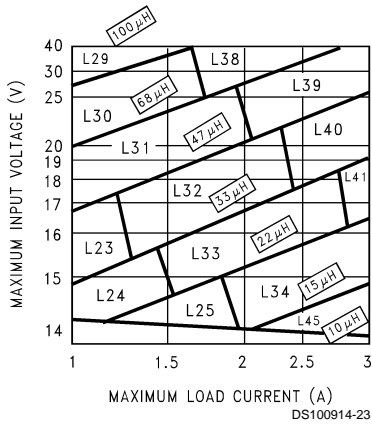
FIGURE 5. LM2676-12
