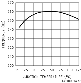
Switching Frequency
