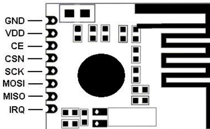
Figure 2 RFM70 pin assignments (top view)
